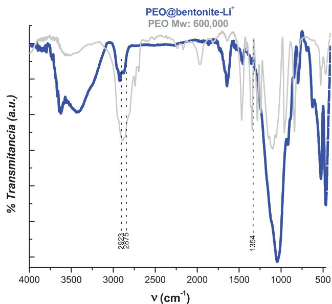
Fig. 2. FT-IR spectra of the polymers and the SPE with PEO@bentonite- \text{Li}^+ with PEO Mw 600,000.
