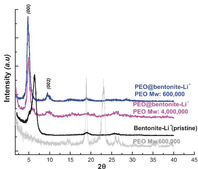
Fig. 1. X-ray diffraction patterns of films of PEO, bentonite- \text{Li}^+ and nanocomposites PEO@bentonite with PEO Mw 600,000 and Mw 4,000,000.
